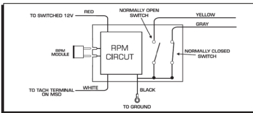
Figure 1 Operation of the RPM Activated Switch.
